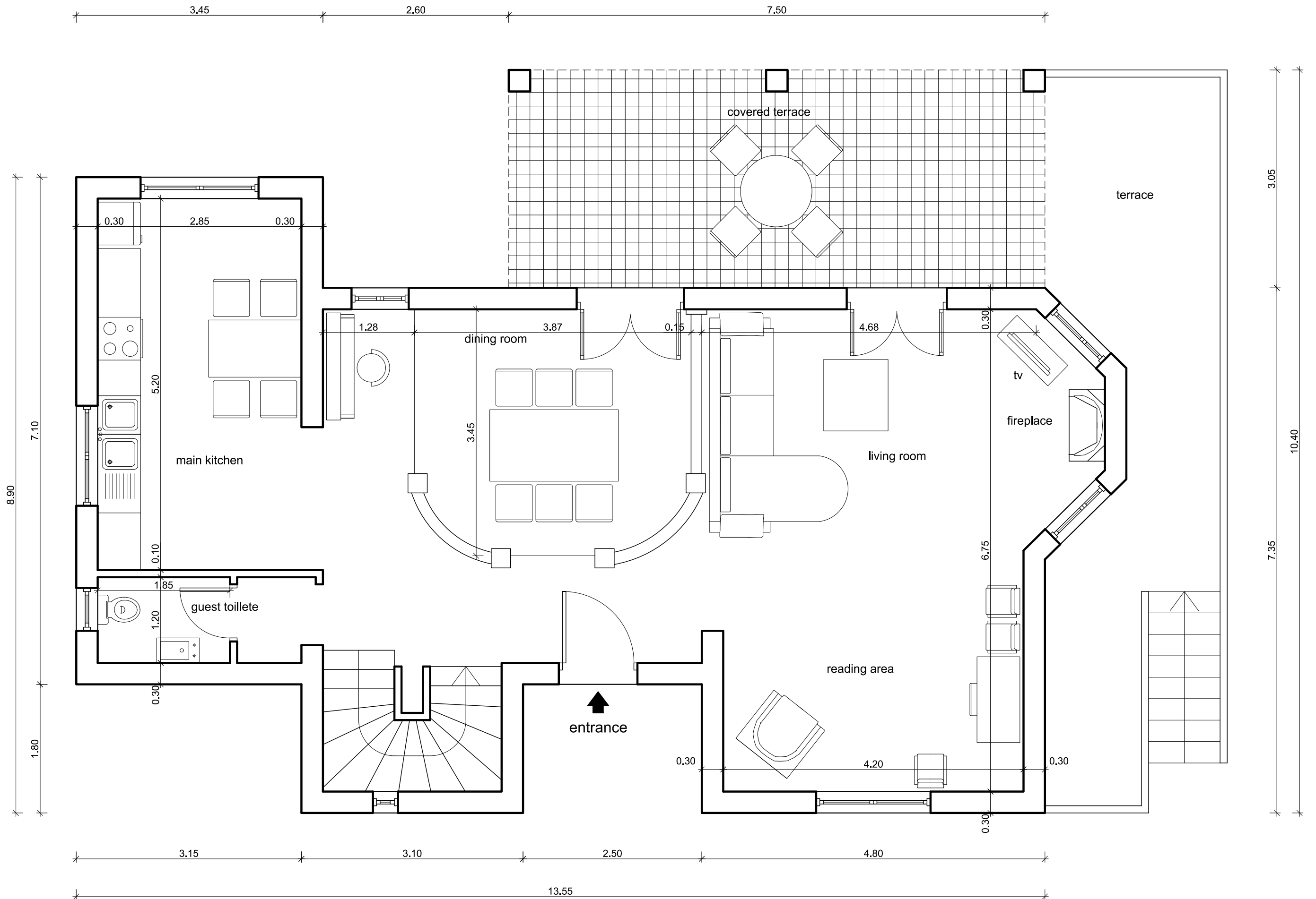
first floor (97,82 m 2 )
