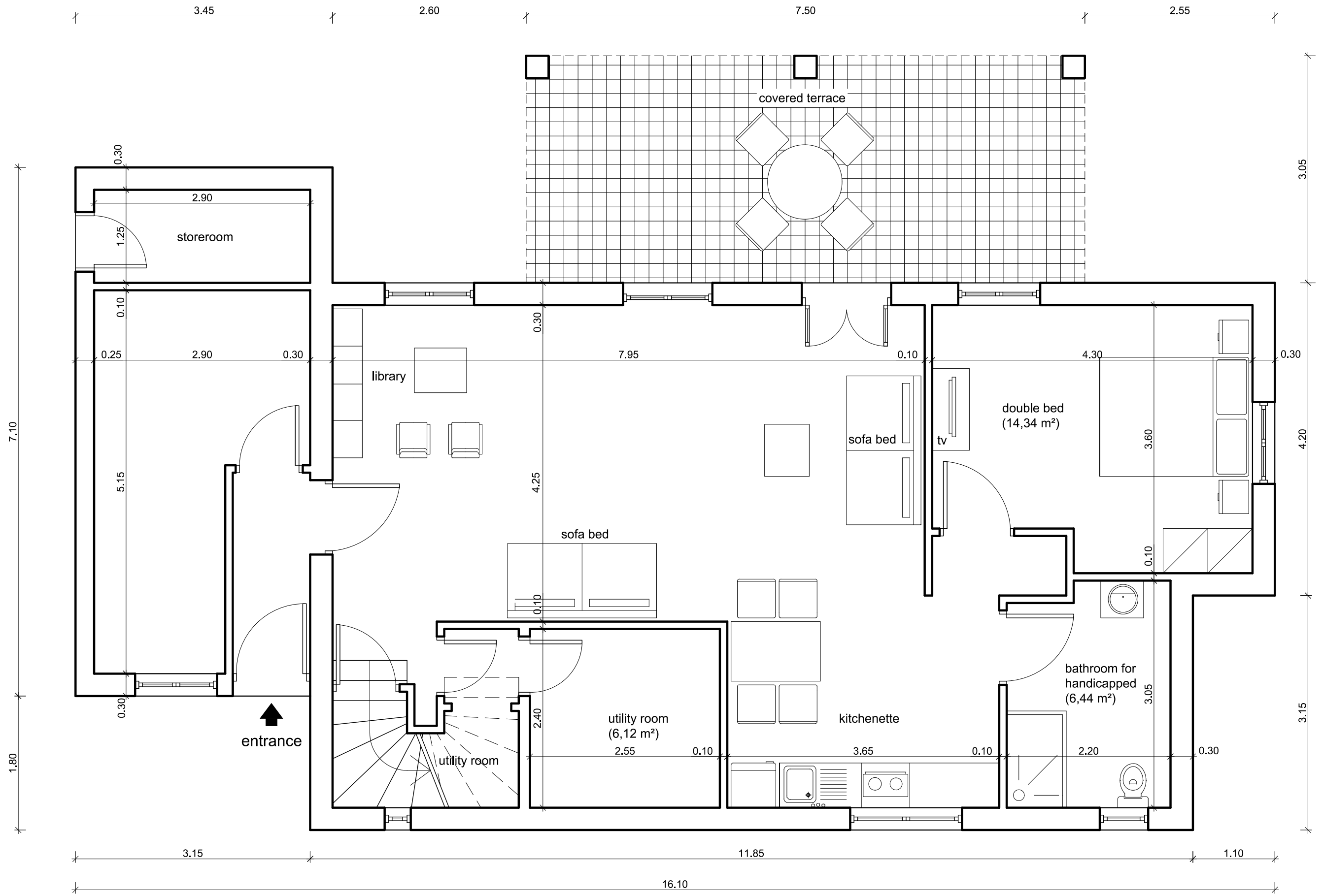
ground floor (114,55 m 2 )
