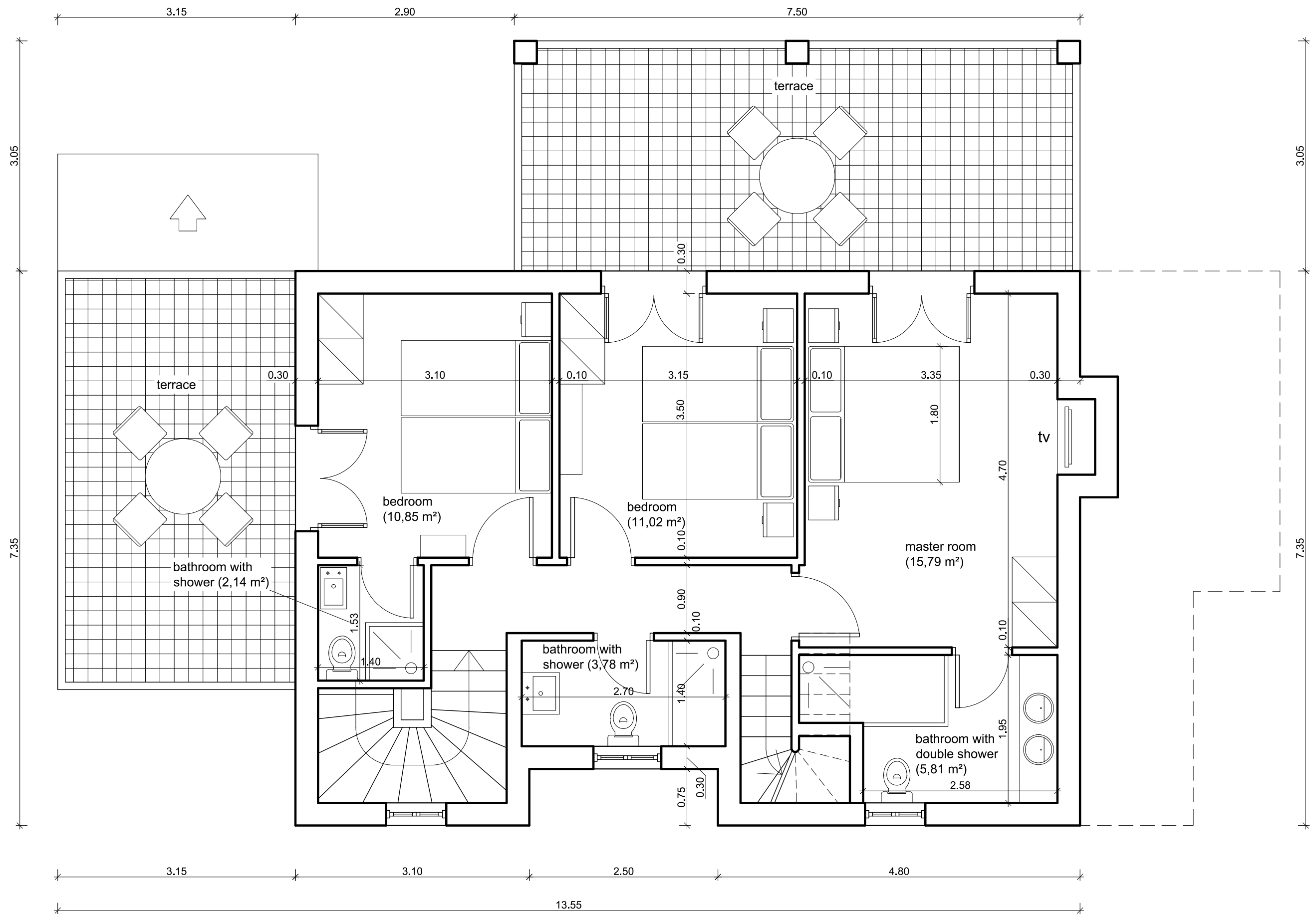
second floor (74,56 m 2 )
